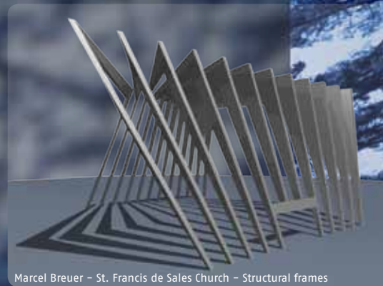
Marcel Breuer – St. Francis de Sales Church – Structural frames
